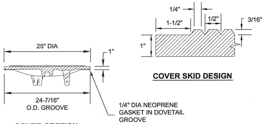
COVER SECTION
